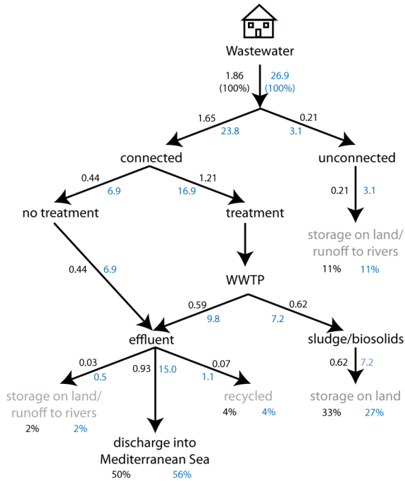
Figure 1. Flowchart for the calculation of direct domestic wastewater discharges of total P (TP) and total N (TN) into the Mediterranean Sea. The numerical values correspond to year 2003 (baseline values) fluxes of P (black) and N (blue) in units of 10 9 mol yr -1 , unless given as percentages of the corresponding total raw wastewater inputs.
